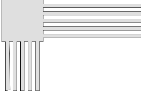
Figure 1: Canonical counterexample
